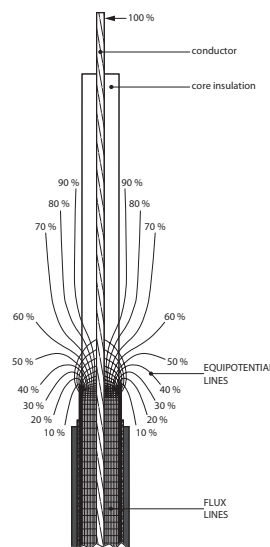
Stress cable
