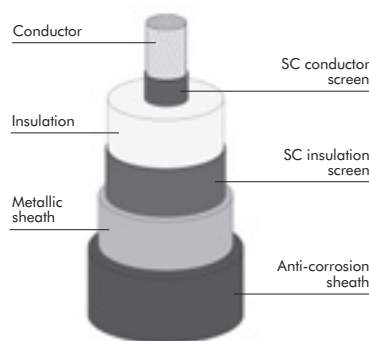
Cable components
