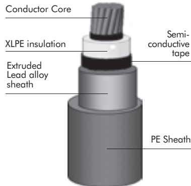
Lead Sheath
